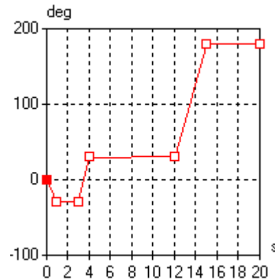
Curve of relative joint angle 2 (drive2)
