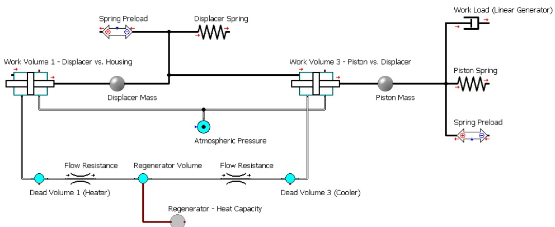
Figure 4: SimulationX model of the free-piston Stirling engine
