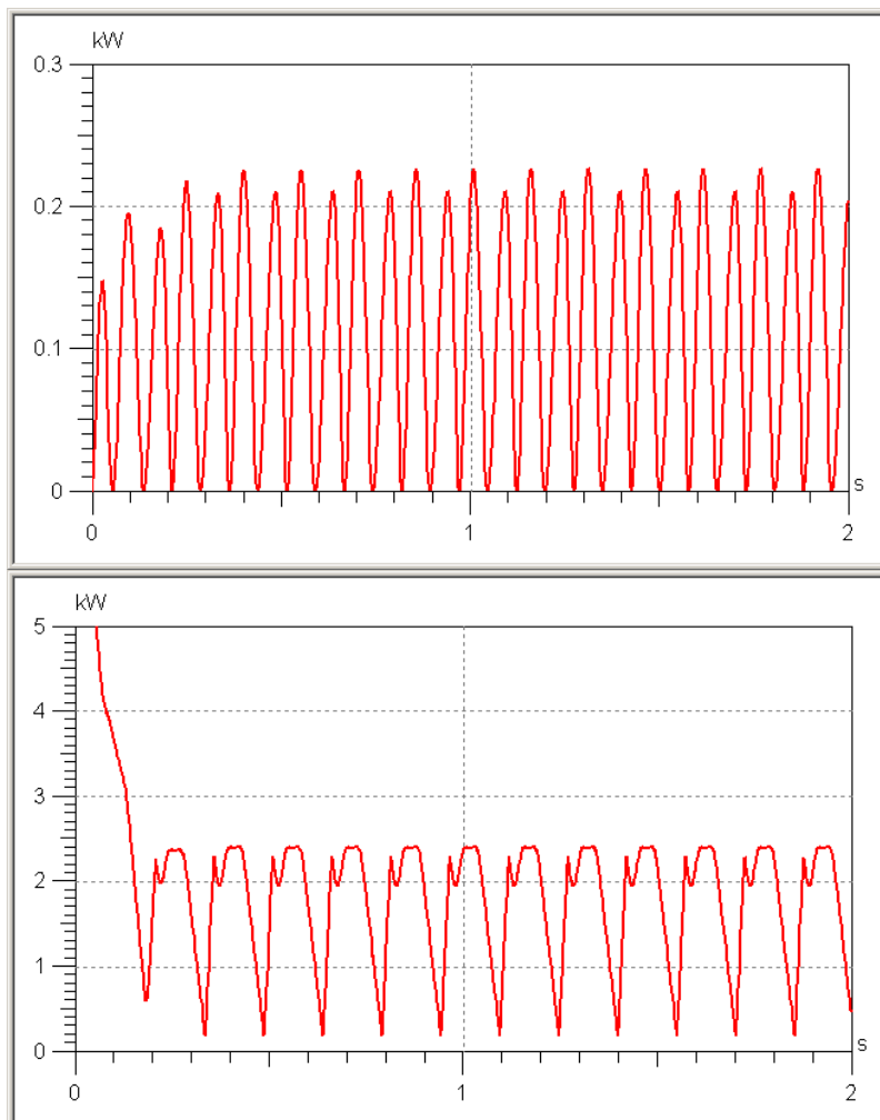
Figure 8: Thermal power input (top) and mechanical power output (bottom)
