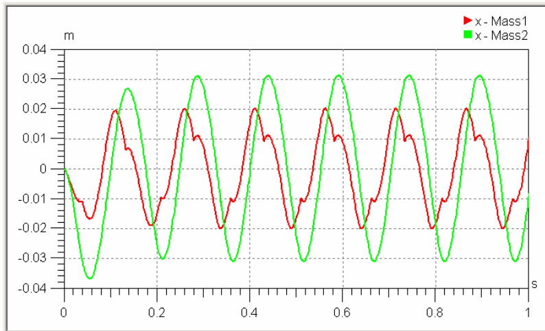
Figure 5: Simulated movement of piston and displacer in the engine (Mass1 – displacer, Mass 2 – piston)
