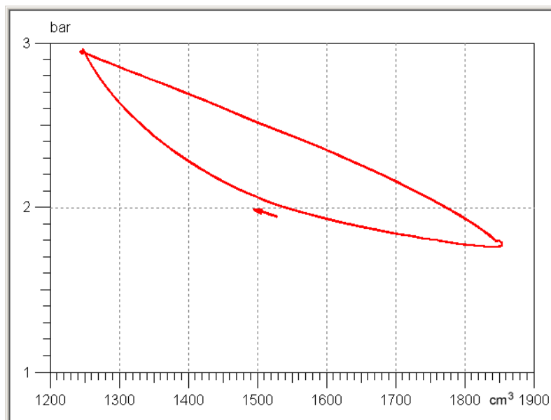
Figure 6: Stirling cycle of the engine model (pressure in the cooler vs. total volume)
