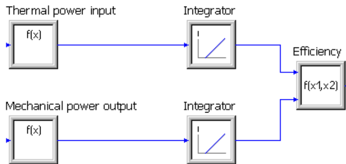
Figure 7: Signal processing structure for the calculation of the engine efficiency
